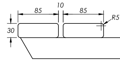
Detail A (1:5)
